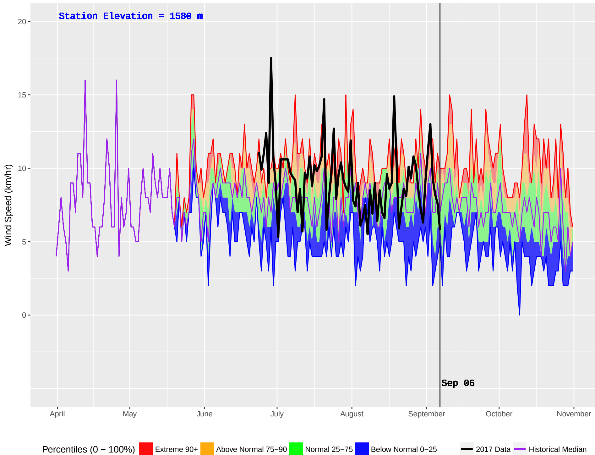
RORY CREEK (1092) : Historical (2010–2016) and Current (2017) Noon Wind Speed
