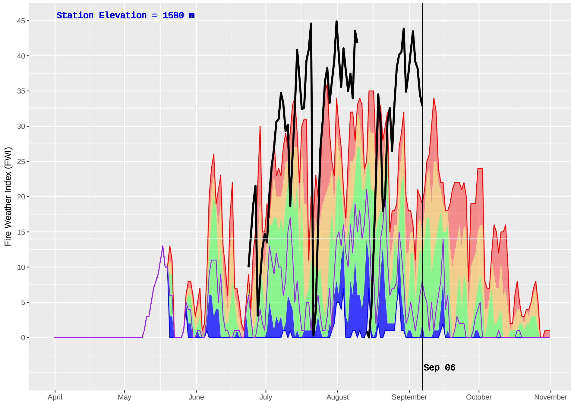
RORY CREEK (1092) : Historical (2010–2016) and Current (2017) Noon Fire Weather Index (FWI)
